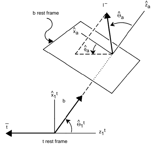
Fig. 4. For the sequential decay t \rightarrow W^+b followed by b \rightarrow l^- \bar{\nu} X , the two pairs of spherical angles \hat{\theta}_1^t, \hat{\phi}_1^t and \hat{\theta}_a, \hat{\phi}_a describe respectively the b momentum in the “first stage” t \rightarrow W^+b and the l^- momentum in the “second stage” b \rightarrow l^- \bar{\nu} X . Angles associated with the b , or \Lambda_b , branching’s momenta directions have “hat” accents whereas those associated with the W^+ branching have “tilde” accents, as in Fig. 7 below. The spherical angles \hat{\theta}_a, \hat{\phi}_a specify the l^- momentum in the b rest frame when the boost is from the t_1 rest frame. In this figure, \hat{\phi}_1^t is shown equal to zero for simplicity of illustration. The positive \hat{x}_a direction is specified by the \bar{t} momentum direction
