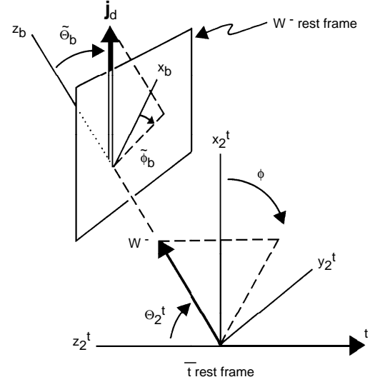
Fig. 8. The labels are as in Fig. 7 but here for the W^- branch. The spherical angles \tilde{\theta}_b, \tilde{\phi}_b specify the j_d jet [or the l^- ] momentum in the W^- rest frame
