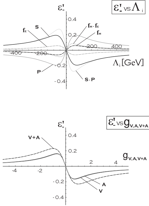
Fig. 11. Plots of the b -polarimetry, \tilde{T}_{FS} -violation, interference parameter \epsilon'_- versus coupling strength for the case of a single-additional pure-imaginary coupling . Curves are for non-gauge-type couplings ( upper plot ), gauge-type couplings ( lower plot ), versus respectively the effective-mass scale \Lambda_i , or coupling strength g_i in g_L = 1 units. Curves are omitted in these plots and in the following Fig. 12 when the couplings produce approximately zero deviations in the helicity parameter of interest
