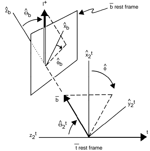
Fig. 5. This figure is symmetric versus Fig. 4. The spherical angles \hat{\theta}_b, \hat{\phi}_b specify the l^+ momentum in the \bar{b} rest frame when the boost is from the \bar{t}_2 rest frame
