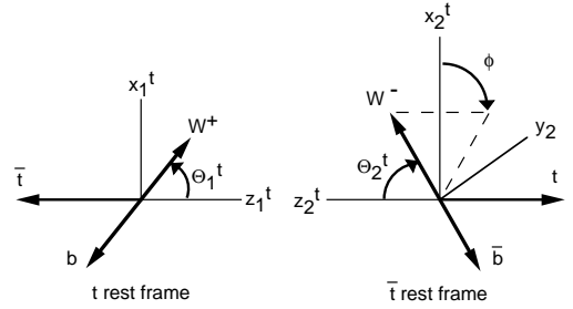
Fig. 3. The three angles \theta_1^t, \theta_2^t and \phi describe the first stage in the sequential-decays of the (t\bar{t}) system in which t \rightarrow W^+ b and \bar{t} \rightarrow W^- \bar{b}
