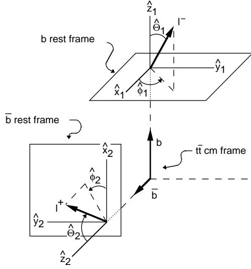
Fig. 6. The spherical angles \widehat{\theta}_1, \widehat{\phi}_1 specify the l^- momentum in the b rest frame when the boost is directly from the (t\bar{t})_{cm} frame. Similarly, \widehat{\theta}_2, \widehat{\phi}_2 specify the l^+ momentum in the \bar{b} rest frame. The b\bar{b} production half-plane specifies the positive \widehat{x}_1 and \widehat{x}_2 axes
