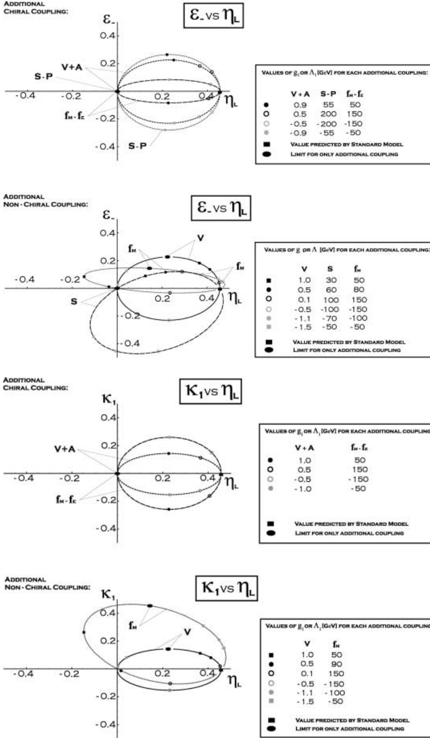
Fig. 9. Plots of the b -polarimetry interference parameter \epsilon_- versus \eta_L for the case of a single-additional, real coupling. The SM prediction is shown by the solid rectangle. The upper plot is for a single-additional, real chiral coupling. The value of \epsilon_- \sim 0 for the other couplings S + P , f_M + f_E . The lower plot is for a single-additional, real non-chiral coupling. The omitted curves for A , P , f_E are respectively almost mirror images about the \eta_L axis. Coupling strengths at representative points are given in the table associated with the respective plot. The unitarity limit is a circle of radius 0.5, centered at the origin, in each of these plots and in those in Fig. 10
