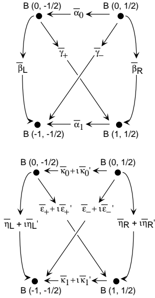
Fig. 2. For \bar{t} \rightarrow W^- \bar{b} decay (the CP -conjugate process), the relative phases and associated helicity parameters are defined as in Fig. 1 but now with “barred” accents. Compare (18–29). Now the R-handed \bar{b} amplitudes, B(\lambda_{W^-}, \lambda_{\bar{b}}) reference the \bar{\alpha}_0, \bar{\alpha}_1 relative-phase-directions, B(\lambda_{W^-}, \lambda_{\bar{b}}) = |B| \exp i\phi_{\lambda_{W^-}^{BR/L}}
