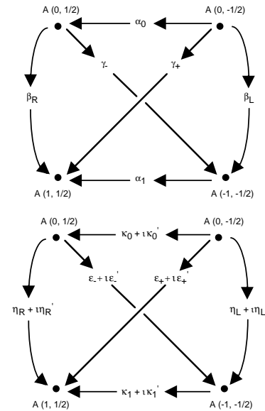
Fig. 1. For t \rightarrow W^+b decay, a display of the four helicity amplitudes A(\lambda_{W^+}, \lambda_b) = |A| \exp(i\phi_{\lambda_{W^+}^L/R}^L/R) relative to the W^+ and b helicities. The upper sketch defines the measurable relative phases and the lower sketch defines their corresponding real-part and imaginary-part (primed) helicity parameters. Throughout this paper the symbol i \equiv \sqrt{-1} . For a pure V - A coupling, the \beta 's vanish and all the \alpha 's and \gamma 's equal +\pi (or -\pi ) to give the overall minus sign in each of the standard model's R-handed b -quark amplitudes, see [12, 13]
