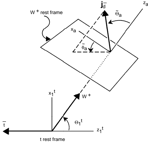
Fig. 7. This figure labels the W^+ branch analogous to the labels in Fig. 4 for the b branch. The two pairs of spherical angles \theta_1^t, \phi_1^t and \tilde{\theta}_a, \tilde{\phi}_a describe the respective stages in the sequential decay t \rightarrow W^+ b followed by W^+ \rightarrow j_{\bar{d}} j_u [or W^+ \rightarrow l^+ \nu ]. The spherical angles \tilde{\theta}_a, \tilde{\phi}_a specify the j_{\bar{d}} jet [or the l^+ ] momentum in the W^+ rest frame
