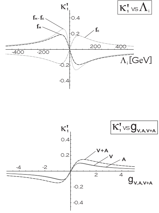
Fig. 12. Plots of the b -polarimetry, \tilde{T}_{FS} -violation, interference parameter \kappa'_1 versus coupling strength for the case of a single-additional pure-imaginary coupling . Curves are for non-gauge-type coupling ( upper plot ), gauge-type coupling ( lower plot ), versus respectively the effective-mass scale \Lambda_i , or coupling strength g_i in g_L = 1 units
